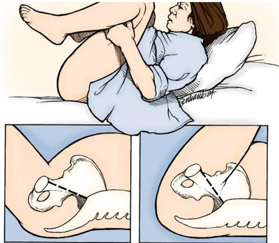
Gambar 3. Manuver McRoberts
