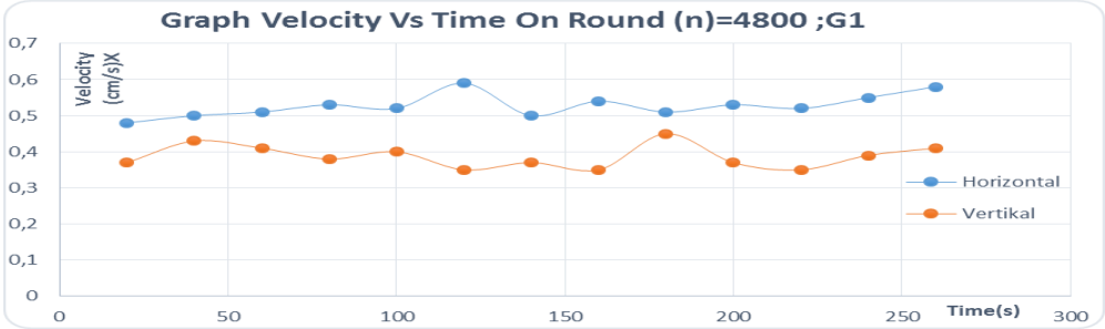
Figure 3.2 Speed relation with time at n = 4800 rpm G1
