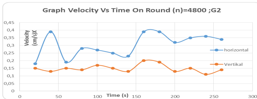
Figure 3.5 Speed with time relationship at n = 4800 rpm, G2
