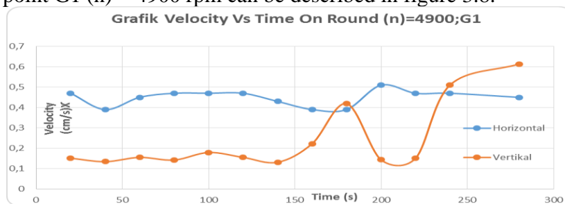
Figure 3.8 Rapid relation with time at n = 4900 rpm G1
