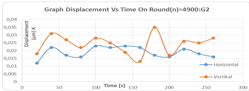
Figure 3.10 The time-drift relationship at n = 4900 rpm G2
