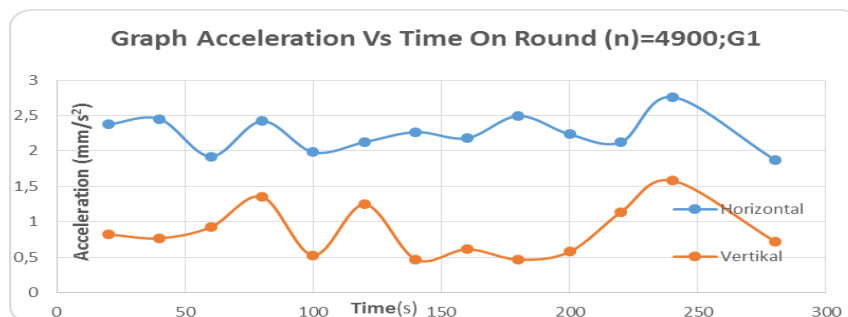
Figure 3.9 Acceleration relationship with time at n = 4900 rpm G1
