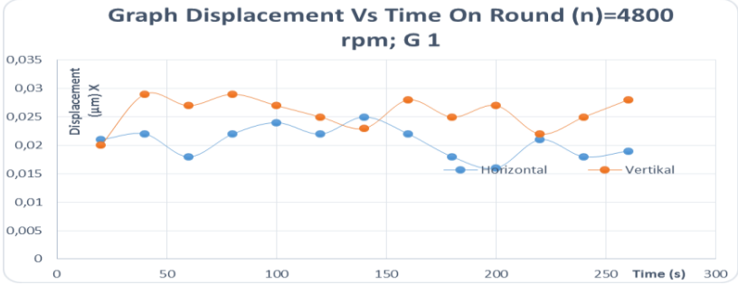
Figure 3.1 The deviation relationship with time at n = 4800 rpm: G1
