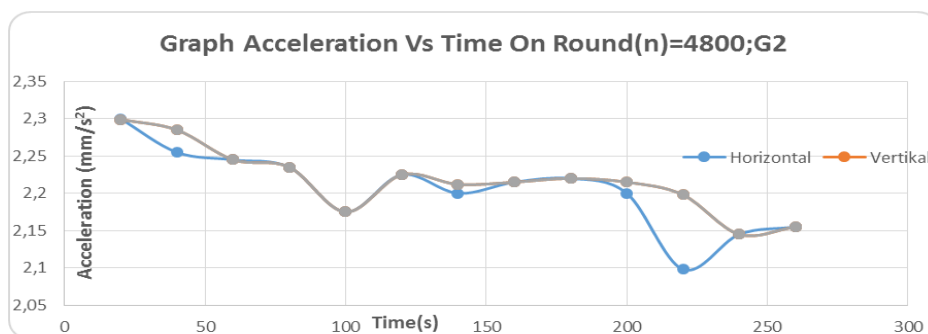
Figure 3.6 Acceleration relationship with time at n = 4800 rpm G2
