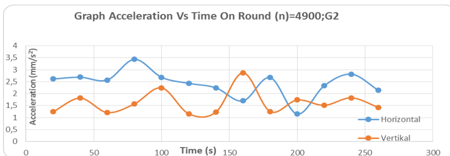
Figure 3.12 Acceleration relationship with time at n = 4900 rpm G2
