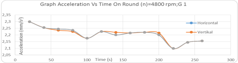
Figure 3.3 Acceleration Relation with Time at n = 4800 rpm G1
