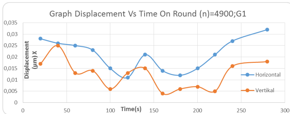
Figure 3.7 The time deviation relationship at n = 4900 rpm G1
