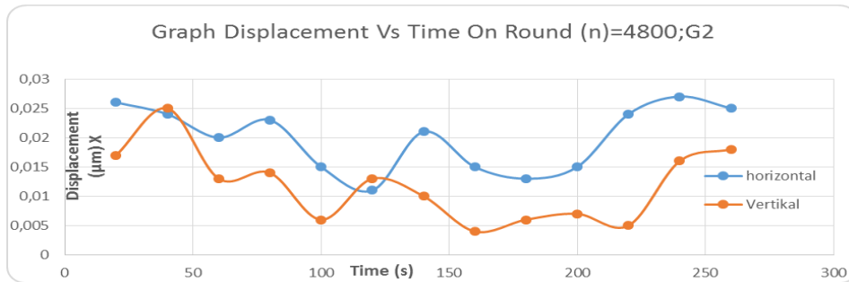
Figure 3.4 The time-drift relationship at n = 4800 rpm: G2
